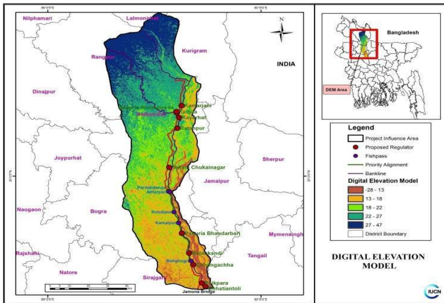
Figure 5.7: Digital Elevation Model (DEM) of the Project Area (Only priority reach to be shown)
