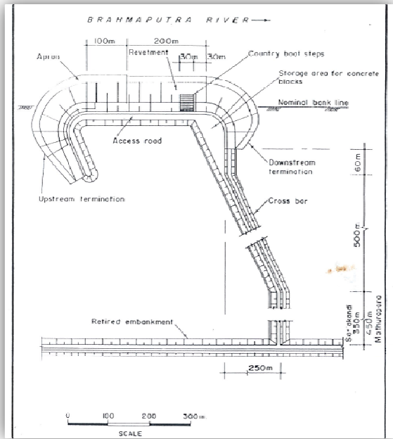
Figure 4.1: Hard Point
