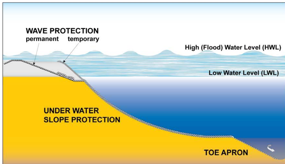
Figure 3.7: The three elements of riverbank protection
