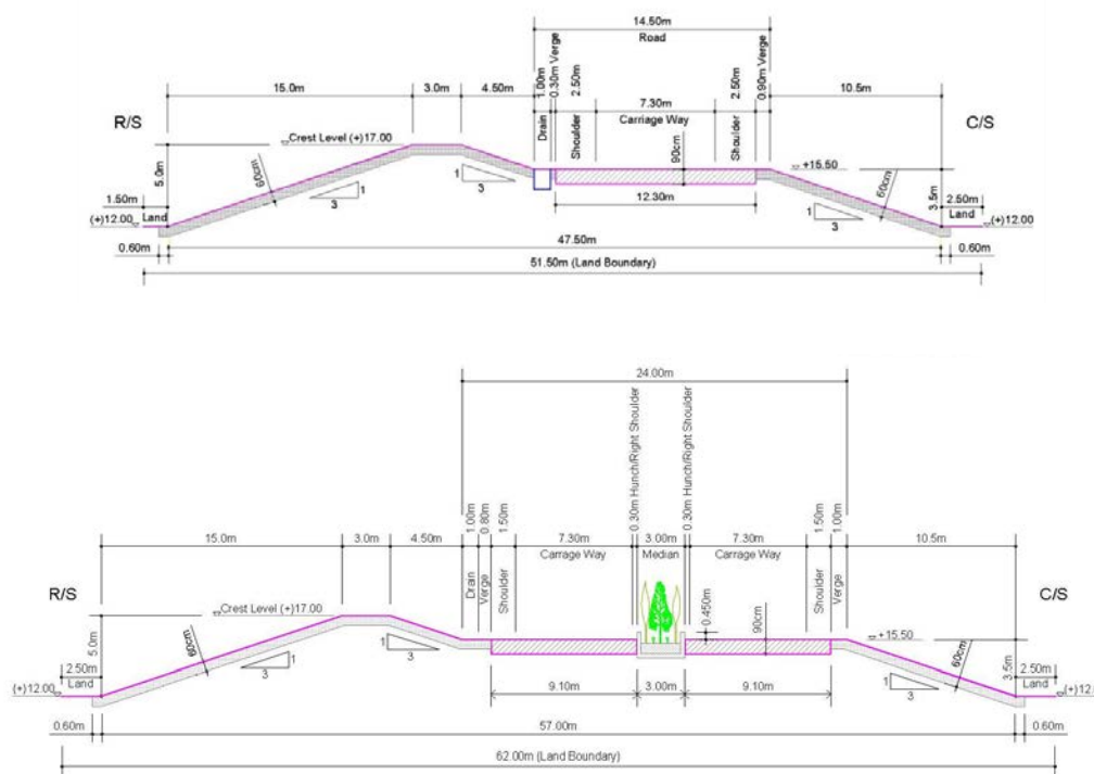
Figure 4.4: Comparison of two- and four-lane road options
