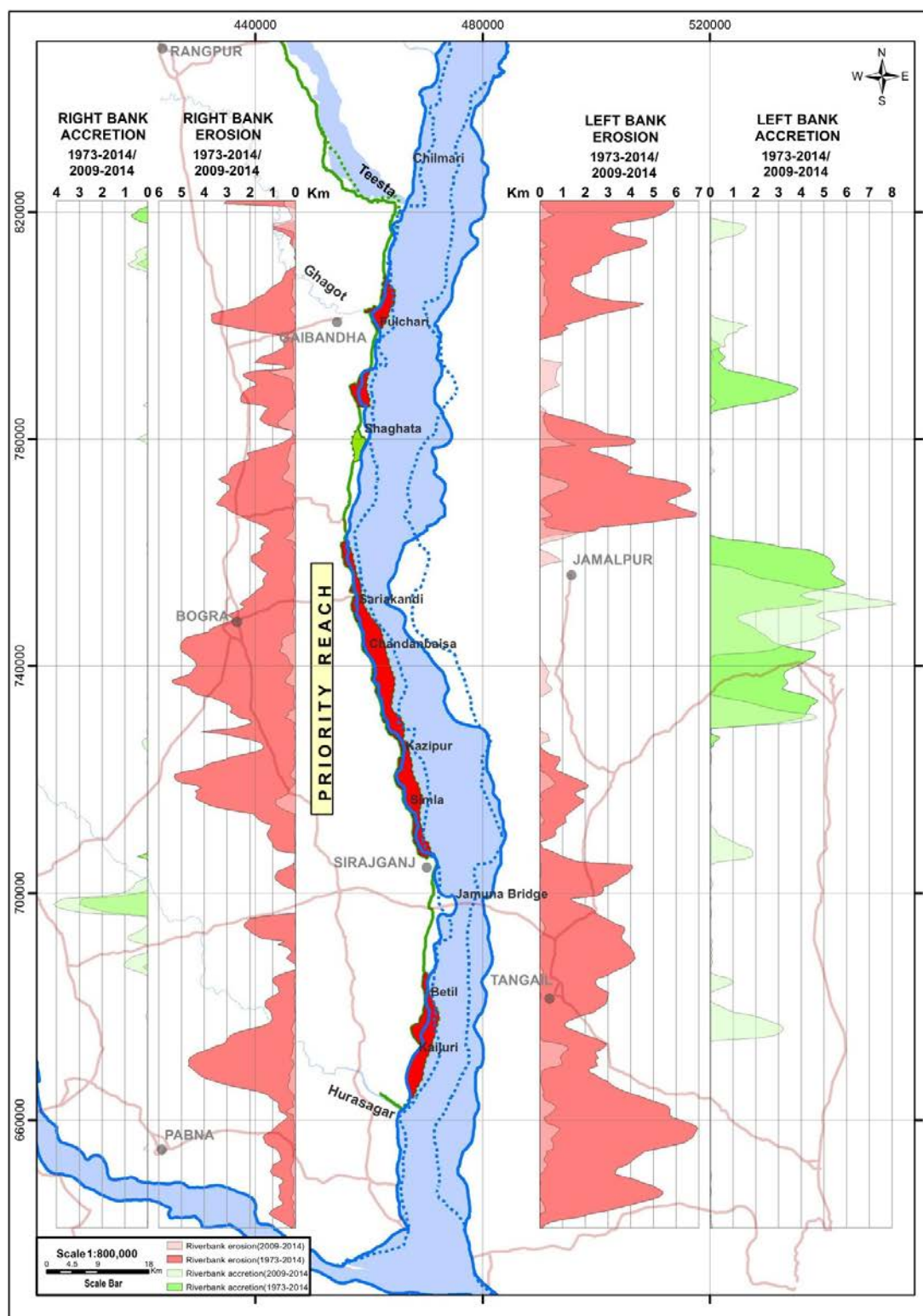
Figure 10.2 Erosion and Accretion of Jamuna from 1973 to 2014
