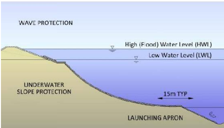
Figure 4.2: Revetment
