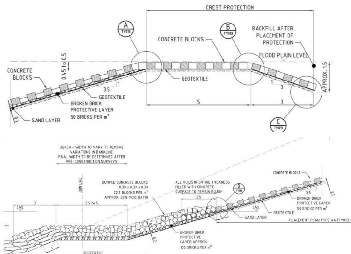
Figure 3.8: Typical cross section of the upper slope treatment
